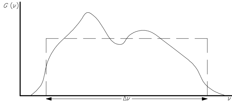
Figure 4.2: A non-flat passband (solid) with an equivalent, flat passband (dashed).
