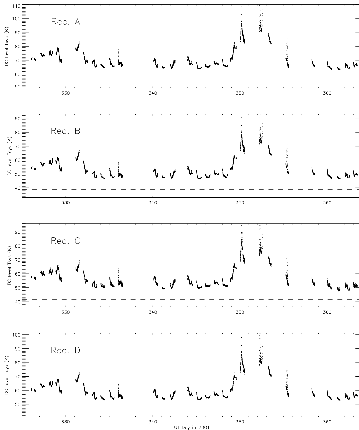
Figure 4.10: T_{sys} vs. time for the 2001 observing campaign. The points are the DC level in each receiver (recorded here once per 200 sec) divided by the average responsivity as measured in the calibration tests. The dashed lines represent the receiver temperature (assumed to be constant through the campaign), also as measured by the average of the calibration tests. The difference between the measured T_{sys} values and the receiver temperature is due to the sky (atmosphere plus \sim 4 K for the C-W corrected and slightly attenuated CMB). All graphs have the same vertical scaling.
