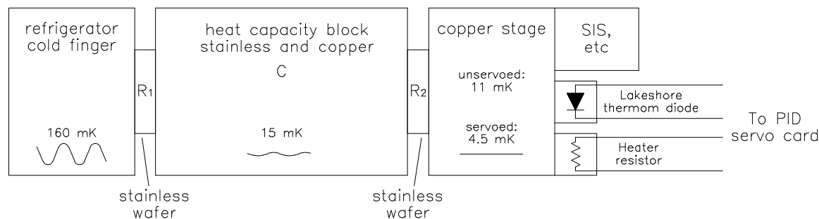
Figure 3.11: Block diagram of the full third-stage cryogenic system. Peak-to-peak thermal variations of a refrigerator cycle, given at several stages along the chain, are from measurements on the fully-assembled receiver A.
