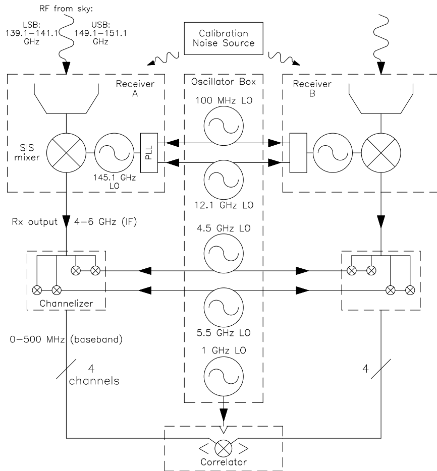
Figure 2.2: The signal path and frequency conversions for a single MINT baseline. The receivers are double-sideband and the correlator is a digital-lag correlator. All oscillators are phase-locked to the 100-MHz source.
