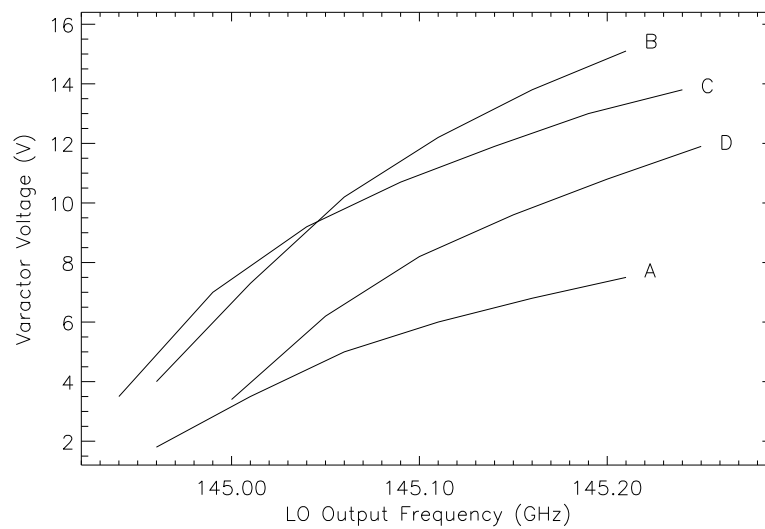
Figure 5.4: Frequency response of the 145.1-GHz LO to varactor voltage. Tuning is a strong function of temperature, which is servoed in the field. For these measurements, the temperature setpoint of the RBE's is 303 K.
