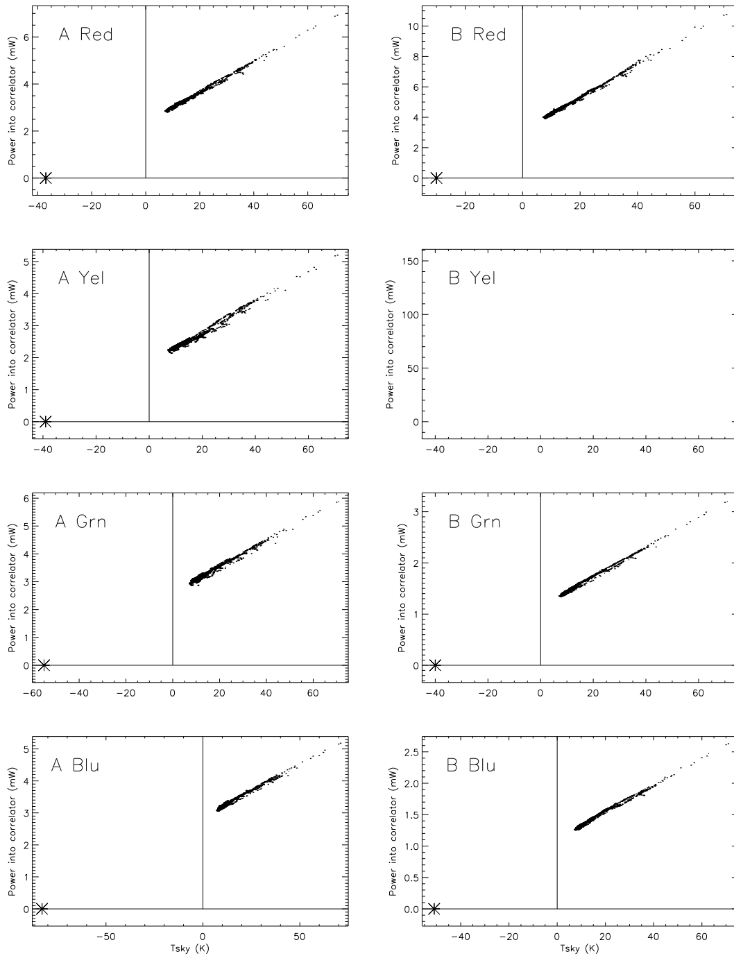
Figure 4.13: Receivers A and B, all channels, power input to correlator vs. sky temperature. In a method analogous to the graphical Y -factor method pictured in Figure 4.1, we calculate T_{rec} (denoted by * ) for each channel using the variable sky as the load. The B-Yellow channel was broken during the campaign.
