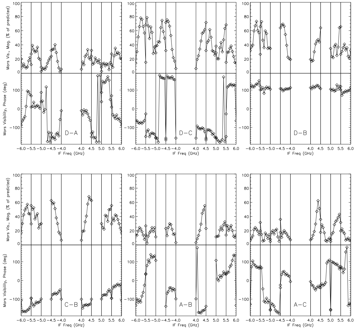
Figure 6.9: Average magnitude and phase of the visibility for Mars. Magnitude is plotted as a fraction of the expected peak signal; since Mars' angular diameter, and thus its antenna temperature, changes through the campaign, we must normalize before averaging. As in the equivalent Jupiter plot (Figure 6.4), data are averaged over the central 1\text{-}\sigma of the cross-beams, so the average magnitude shown in this plot is lower than that quoted in Table 6.5.
