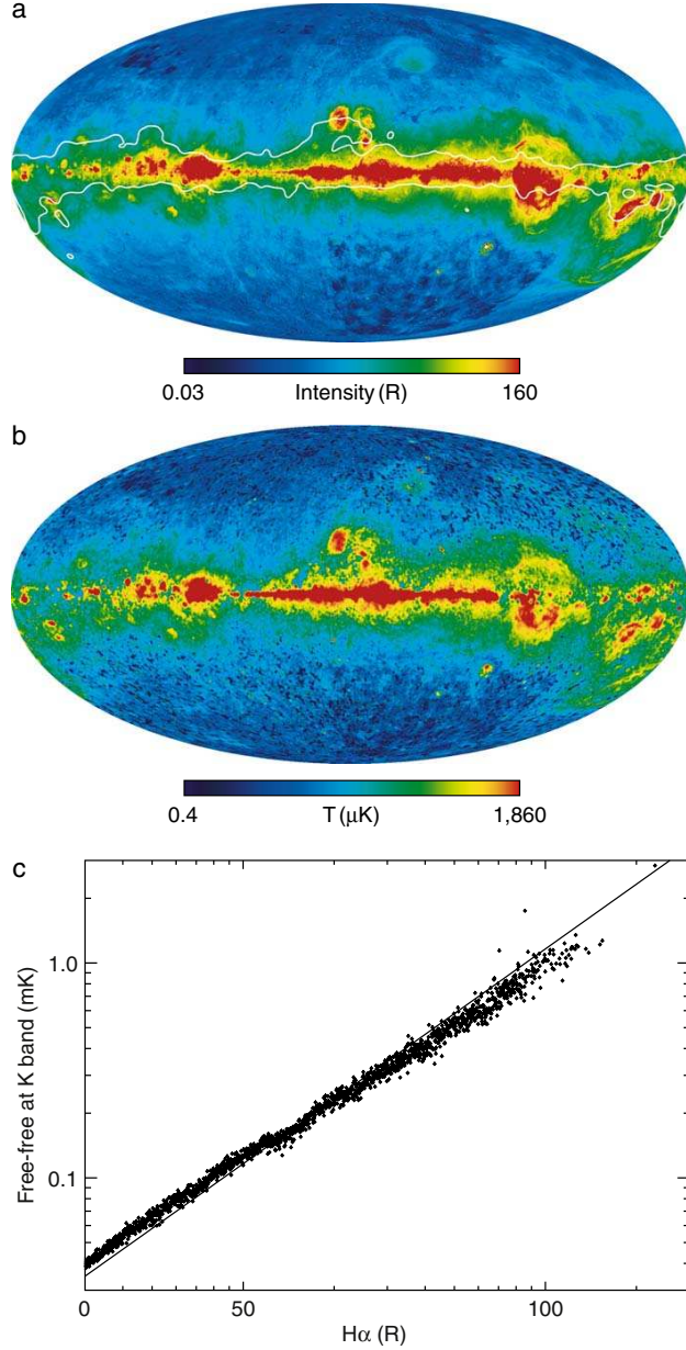
Fig. 3.— (a) A H \alpha map of the sky, corrected for extinction. The correction is only an approximation and is especially unreliable for regions where \tau > 1 . These high opacity regions are roughly demarcated by the contour lines, which have been smoothed for clarity. (b) A full sky map of free-free emission based on the five bands of WMAP measurements. The map is the result of the MEM modeling process, as described in the text. (c) Pixel values in the MEM-derived free-free map are compared against their values in the H \alpha map, with each point representing an average in H \alpha intensity bins of \Delta I = 8 R . The lack of scatter in the fainter bins reflects fidelity to the prior assumption of 11.4 \mu\text{K}/R at K-band. The data plotted only includes pixels where the H \alpha optical depth is estimated to be < 0.5 and the K-band antenna temperature is > 0.2 mK. The data are consistent with the \mu\text{K}/R values given in Table 1 within \sim \pm 12\% uncertainty, depending on the fitting method used.
