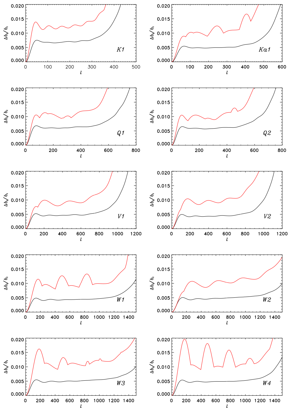
Fig. 11.— Relative error in beam transfer functions ( \Delta b_\ell/b_\ell ) for the five-year beams (black) vs. the three-year errors (red) (Jarosik et al. 2007). The five-year uncertainties are typically a factor of \sim 2 better than three-year uncertainties.
