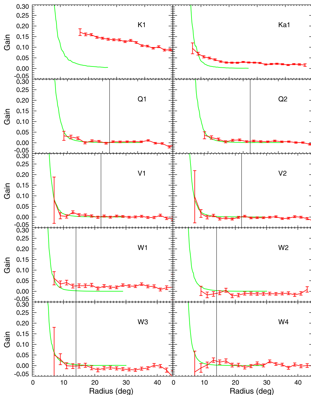
Figure 6. A-side augmented beam profiles (green) compared to Moon sidelobe data (red). K1 and Ka1 appear to be dominated by diffuse reflection rather than the extended main beam, and so are excluded from the fit. Conspicuous DA-to-DA differences are seen in the quality of the fit, e.g., W1 and W2 as compared to V1 and V2. Contamination of the fit by diffuse reflected light cannot be ruled out even in DAs other than K1 and Ka1; thus, the Moon data are best considered as upper limits. Vertical line: maximum radius of Moon data included in fit, for DAs Q1–W4.
