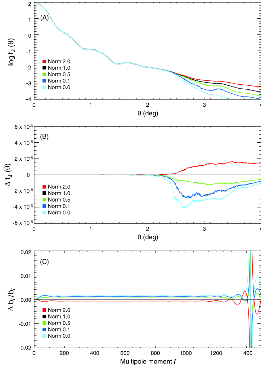
Figure 9. Top: radially binned noise-free simulations of hybridized beams for the V2 DA. The central part of the beam is taken from the adopted DADRA model without augmented distortions. The part of the beam below a given gain cutoff is taken from augmented beam models with various normalizations of the extrapolated primary-mirror distortions. The analysis of hybrid beams including real Jupiter data favors the zero normalization, meaning that the extrapolated distortions are omitted. Middle: same profiles as in the top panel, after subtraction of the one with normalization 1.0. Bottom: beam transfer functions corresponding to the depicted beam profiles, relative to the one with normalization 1.0. Fits using flight hybrid beams should approximate the curves shown here.
