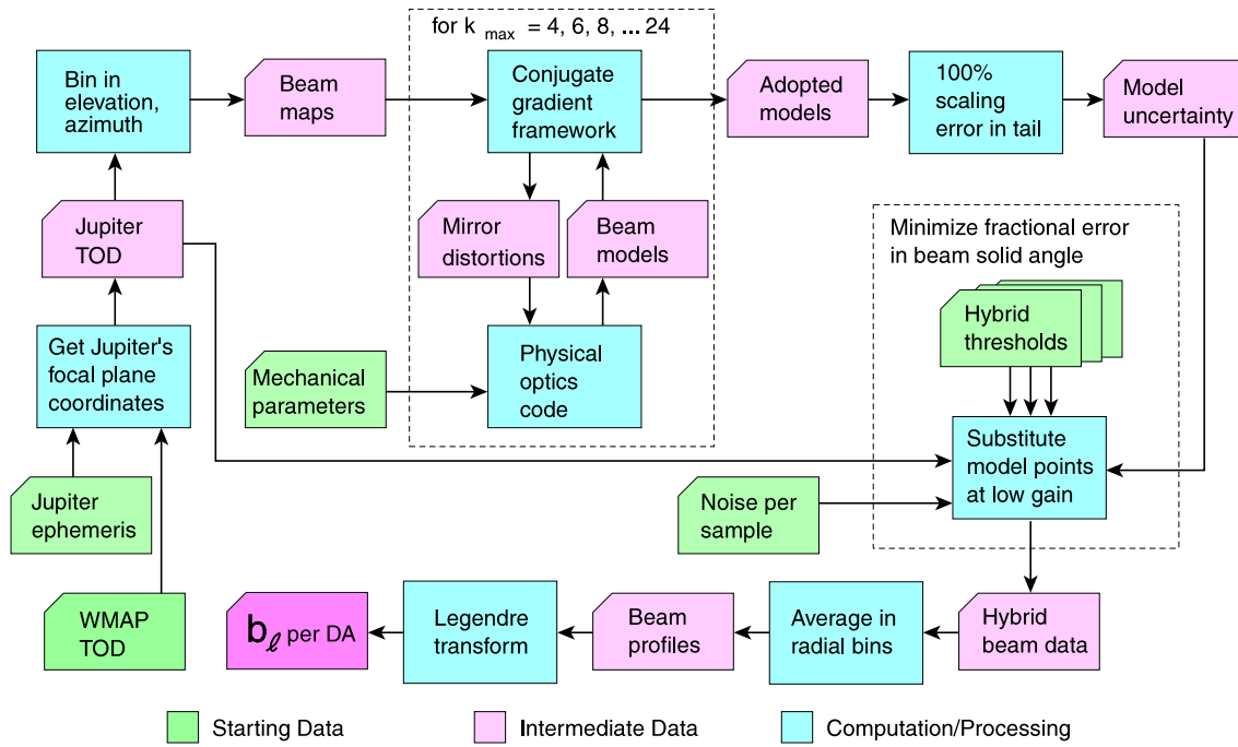
Figure 1. Flow chart of beam and window function processing. Boxes are color coded as follows: green , starting data; pink , intermediate data; blue , computations or processing steps; magenta , the result, b_\ell , which is the beam transfer function. The window function, w_\ell , for power spectra C_\ell involving a single DA, is b_\ell^2 . Dashed boxes enclose iterative algorithms.
