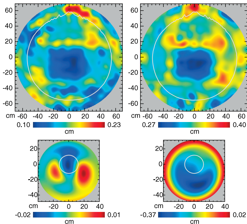
Figure 3. Fitted distortions of the A-side (left) and B-side (right) mirrors with respect to nominal shapes. Y axis is negative in the sky direction and positive toward the main spacecraft structure. Top row: primary mirrors. The dominant feature of the primary mirror distortions is the central rectangle, corresponding to a frame that is part of the backing structure. Hints of the stiffening lugs in the backing structure may also be seen around the edges. Bottom row: secondary mirrors. The mirrors are constrained only where they are substantially illuminated by the feed horns (Page et al. 2003b). Thus, for example, the secondary mirror for the B side appears as a bullseye partly because the fit is only constrained near the center. Gray line: contour of the mean W-band illumination function -15 dB from the peak. Although the mirrors are elliptical in outline, these plots are circular. The reason is that the distortions are parametrized as displacements along the axis of a circular cylinder containing the mirror boundary.
