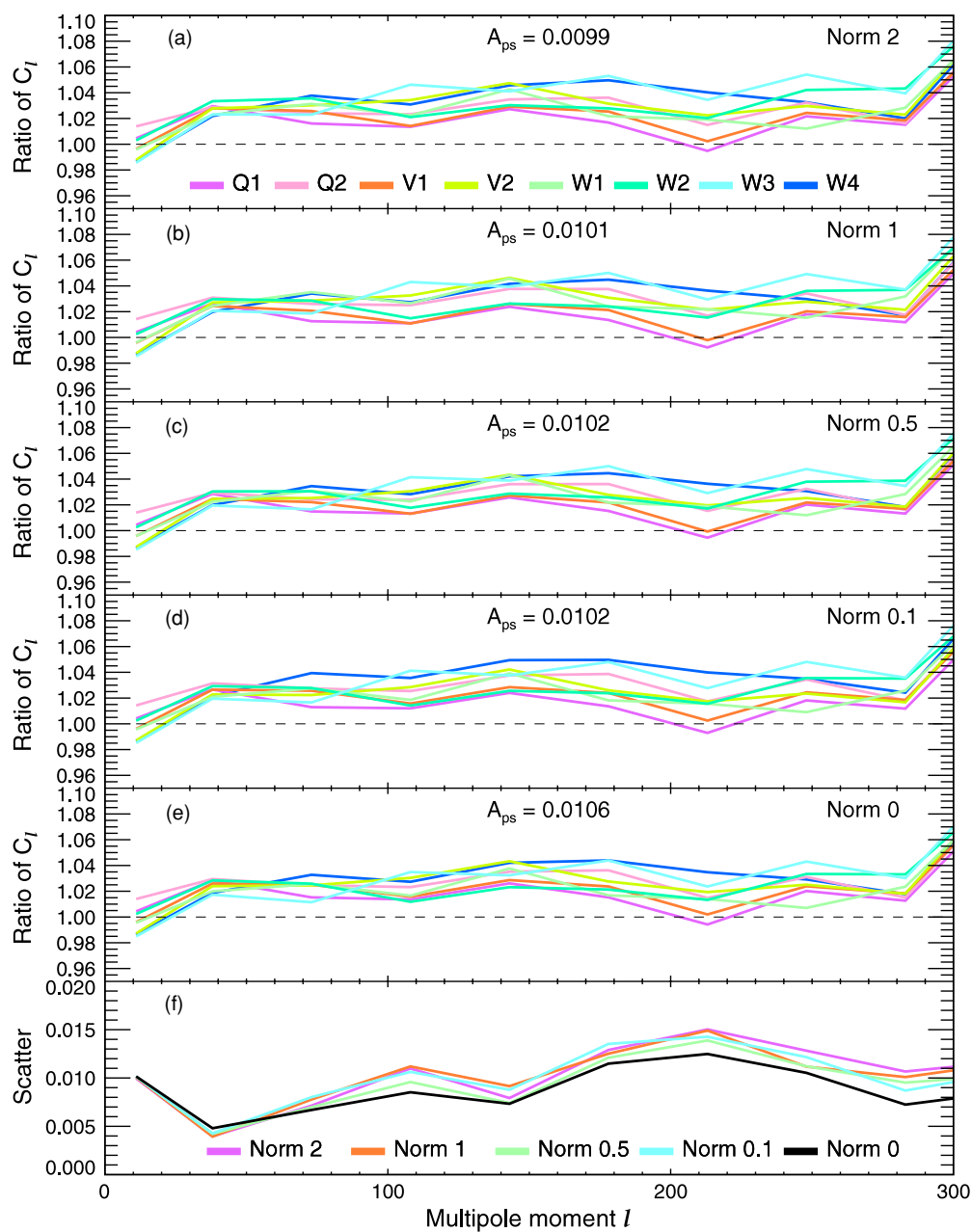
Figure 10. Consistency of CMB power spectra across frequency bands, for window functions derived from various normalizations of the extrapolated primary mirror distortions. Complete omission of such extrapolated distortions from the main beam model is justified by this criterion. The CMB spectra and unresolved point-source coefficients ( A_{ps} ) in this plot are from a preliminary stage of analysis and are not the final five-year WMAP results. (a)–(e): Mean of year-to-year cross spectra in each DA, relative to the final combined power spectrum from the three-year analysis. The applied w_\ell are derived from hybridized beams in which the tail is from a beam model with extrapolated primary mirror distortions; hybridization thresholds in each DA optimize solid angle error for the nominal amplitude of these added distortions (Figure 5). Spectrum is binned in l with a bin size of \Delta l = 35 . The panels differ in the scaling of the extrapolated distortion amplitude on the mirror: (a), 2; (b), 1; (c), 0.5; (d), 0.1; (e) no extrapolated distortions. (f) Scatter among the DAs in each l bin for the five normalizations of the extrapolated mirror distortions. Omitting the extrapolated distortions (Norm 0, black) minimizes the scatter in the CMB power spectrum over most of this l range, which includes the first peak near l \sim 200 .
