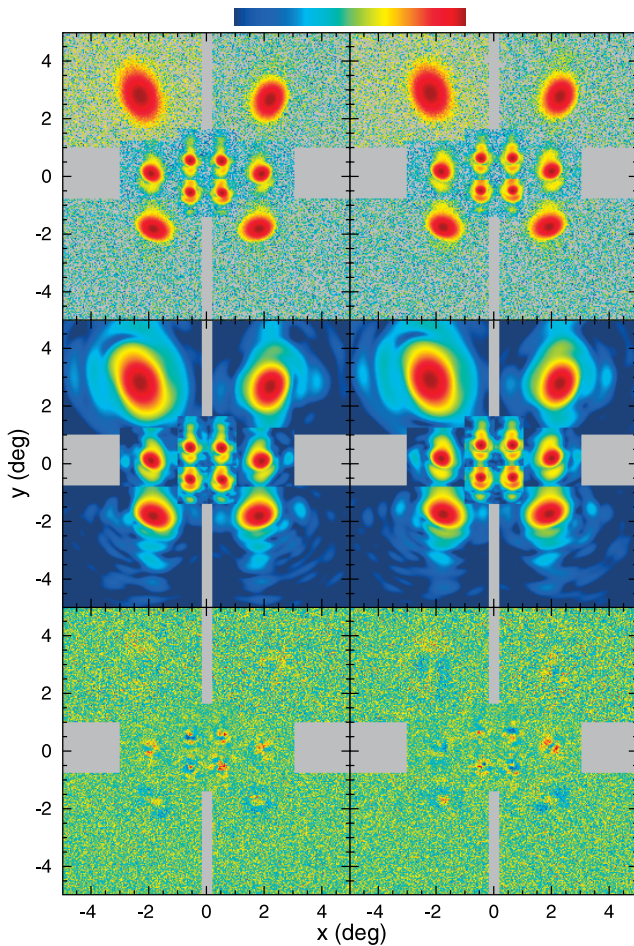
Figure 2. Beams in the WMAP focal plane for side A (left) and side B (right). The top panels show the measured beams, the middle panels show the beam models, and the bottom panels show the residuals. In the top four panels, each beam is scaled to its maximum (red) and plotted logarithmically to a level of -40 dB (blue). For the bottom panels, each beam's residual is shown linearly as 100(\text{data} - \text{model})/\text{beam peak} . The scales are \pm 10\% for K1, \pm 5\% for Ka1, Q1, and Q2, \pm 3\% for V1 and V2, and \pm 2.5\% for W1–W4. A similar depiction of the A side only for three years of data is in Figure 9 of Jarosik et al. (2007).
