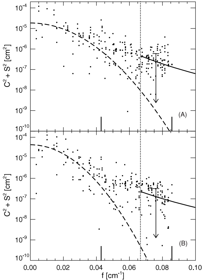
Figure 5. Power spectra of A-side (top) and B-side (bottom) primary mirror distortions as a function of spatial frequency on the primary mirror surface, f = k/(280 \text{ cm}) , where k is the spatial frequency index used in the physical optics fits. Vertical bars on the f axis indicate f corresponding to k = 12 and k = 24 . Solid lines: extrapolated power-law distortion spectra with slopes fitted by comparison to Moon sidelobe data, namely, \alpha = 4.95 for the A side and \alpha = 4.43 for the B side. In practice, these extrapolated distortions are used to update the sidelobe response patterns, but not to model the main beams. The error bars and upper limits show the mean absolute deviation about the mean of points with length scales less than 15 cm, indicated by the dotted vertical line. Dashed curves: power spectra of primary mirror distortions from ground-based laboratory measurements of the surface, assuming a Gaussian form for the two-point correlation function, with correlation length 9.3 cm for the A side and 11.3 cm for the B side; normalized to points with f < 0.05 \text{ cm}^{-1} (top) and f < 0.04 \text{ cm}^{-1} (bottom).
