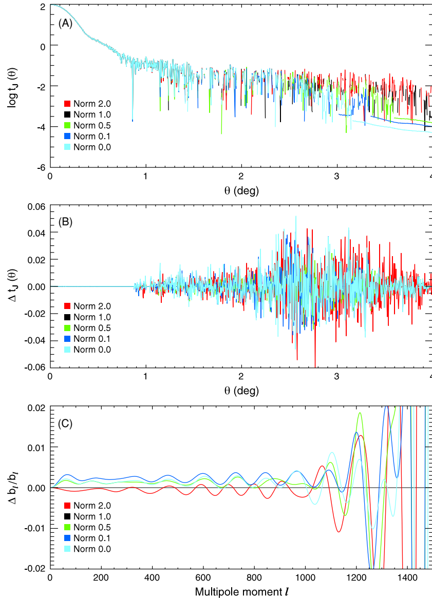
Figure 8. Top: symmetrized radial profiles of hybridized, binned flight beams for the V2 DA. The central, high S/N part of the beam is taken directly from flight data of the planet Jupiter, whereas the part of the beam below a given gain cutoff is taken from beam models. The set of beam models shown comprises several normalizations of the extrapolated primary-mirror distortions; the normalization favored in the analysis is zero, meaning that the extrapolated distortions are omitted. The noise-free lines at radii 3^\circ – 4^\circ are portions of the lower-normalization profiles that include model points only. Middle: same profiles as in the top panel, after subtraction of the one with normalization 1.0. Bottom: beam transfer functions corresponding to the depicted beam profiles, relative to the one with normalization 1.0. Cf. Figure 9, especially the bottom panel. The beam transfer functions at \ell \gtrsim 100 are close to what is expected from the noise-free simulations, implying good solid angle recovery.
