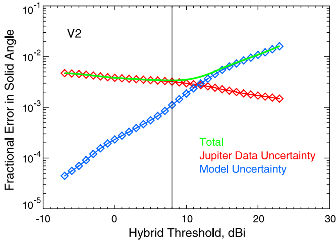
Figure 7. Fractional error in hybrid beam solid angle as a function of hybridization threshold, for the V2 DA. As the hybridization threshold is raised, noisy Jupiter data are excluded, so that the Jupiter data uncertainty (red) falls. At the same time, the model uncertainty (blue), estimated as a scaling error of 100%, increases because more of the two-dimensional model beam is used. These contrary slopes produce a well defined minimum in the total error (green). Hybridization threshold values for the five-year analysis are chosen near the location of this minimum, as shown by the vertical line. Plots for other DAs are similar. The adopted thresholds are rounded to an even dBi unit and are constant for each frequency band, as shown in Table 3.
