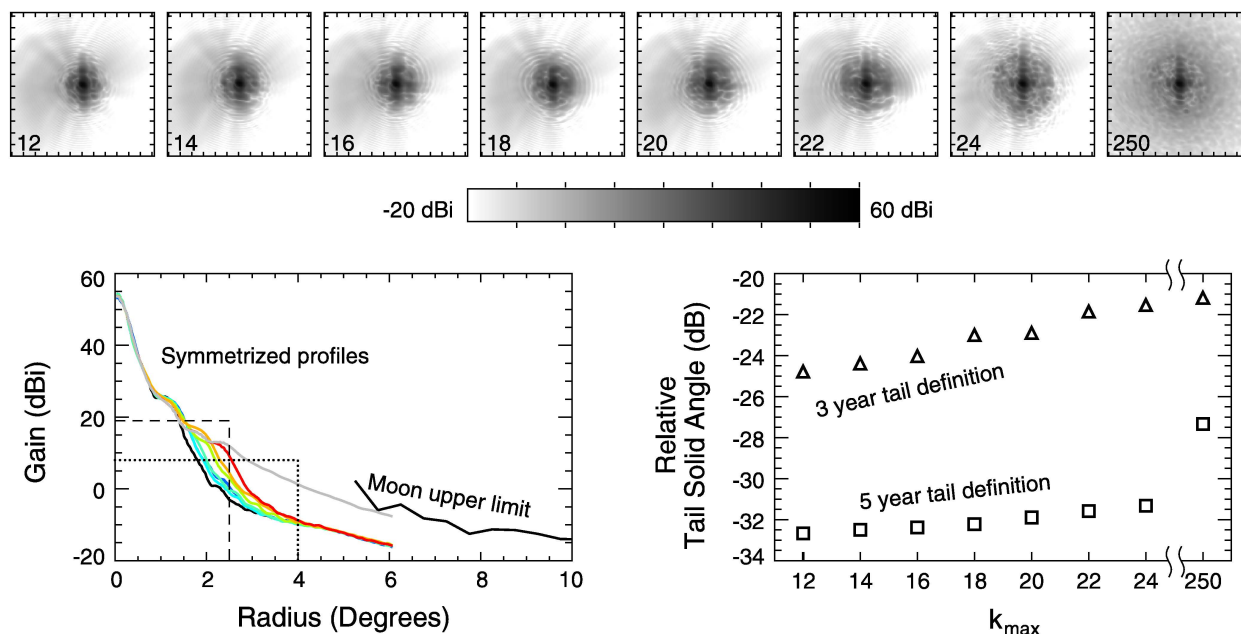
Figure 4. Growth of solid angle in model beams as a function of k_{\max} , for the V2 DA on the A side. Top: logarithmically scaled images of the model beam pattern as fitted for k_{\max} = 12, 14, 16, 18, 20, 22, and 24 , respectively, together with a beam that combines the k_{\max} = 24 fit with random-phase modes extrapolated to k = 250 . Axis tick marks are at 1^\circ intervals. Bottom left: azimuthally averaged beam profiles for the models pictured, in units of gain relative to isotropic. Indigo-red: profiles of the seven beam models from k_{\max} = 12 through k_{\max} = 24 , respectively. Gray: k_{\max} = 250 extrapolation result. Black: upper limit on the main beam sensitivity from Moon observations, obtained for side A by integrating over positive pixels in the differential sidelobe response pattern. The five-year model tail, which is a feature of the two-dimensional beam pattern, is the part of the beam that is both inside the transition radius and below the hybridization threshold (dotted line; see Section 3.3). The hybridization threshold and transition radius from the three-year analysis are indicated by the dashed line. Bottom right: model tail solid angle as a function of k_{\max} , relative to the total solid angle inside the transition radius; squares, five-year; triangles, modified tail of five-year models, using three-year threshold and transition radius. Fitting to k_{\max} = 24 rather than k_{\max} = 12 increases by a factor of \sim 2 the solid angle of the model tail as defined by three-year main beam limits. But note that the difference between the various fits is \sim 0.1\% of the total beam solid angle for the 5 year data.
