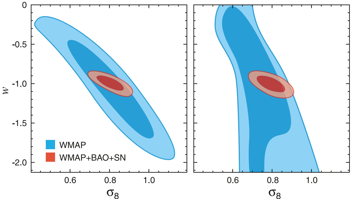
FIG. 16.— Predictions for the present-day amplitude of matter fluctuations, \sigma_8 , as a function of the (constant) dark energy equation of state parameter, w , derived from the full WMAP data (blue) as well as from WMAP+BAO+SN (red). The contours show the 68% and 95% CL. (Left) Flat universe, \Omega_k = 0 . (Right) Curved universe, \Omega_k \neq 0 .
