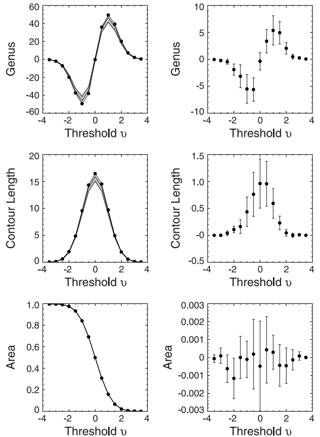
FIG. 7.— Minkowski functionals from the WMAP 5-year data, measured from the template-cleaned V+W map at N_{\text{side}} = 128 (28' pixels) outside of the KQ75 mask. From the top to bottom panels, we show the Euler characteristics (also known as the genus), the contour length, and the cumulative surface area, as a function of the threshold (the number of \sigma 's of hot and cold spots), \nu \equiv \Delta T/\sigma_0 . (Left) The data (symbols) are fully consistent with the mean and dispersion of Gaussian realizations that include CMB and noise. The gray bands show the 68% intervals of Gaussian realizations. (Right) The residuals between the WMAP data and the mean of the Gaussian realizations are highly correlated from bin to bin. From this result we find f_{NL}^{\text{local}} = -57 \pm 60 (68% CL). From N_{\text{side}} = 64 we find f_{NL}^{\text{local}} = -68 \pm 69 (68% CL).
