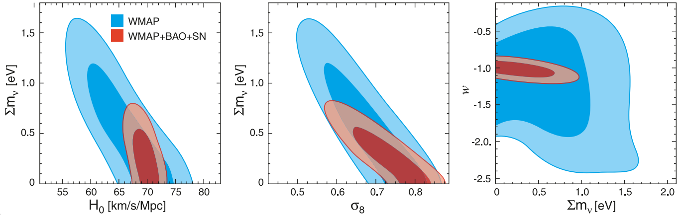
FIG. 17.— Constraint on the total mass of neutrinos, \sum m_\nu (§ 6.1.3). In all panels we show the WMAP-only results in blue and WMAP+BAO+SN in red. (Left) Joint two-dimensional marginalized distribution of H_0 and \sum m_\nu (68% and 95% CL). The additional distance information from BAO helps reduce the correlation between H_0 and \sum m_\nu . (Middle) The WMAP data, combined with the distances from BAO and SN, predict the present-day amplitude of matter fluctuations, \sigma_8 , as a function of \sum m_\nu . An independent determination of \sigma_8 will help determine \sum m_\nu tremendously. (Right) Joint two-dimensional marginalized distribution of w and \sum m_\nu . No significant correlation is observed. Note that we have a prior on w , w > -2.5 , and thus the WMAP-only lower limit on w in this panel cannot be trusted.
