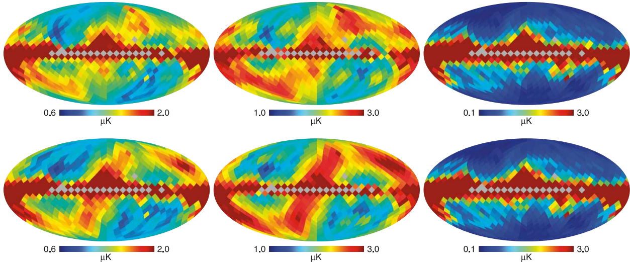
Fig. 2.— Estimated 1\sigma errors on the low resolution maps of the CMB (left), synchrotron (center), and dust (right) Q and U components, as shown in Figure 1. The CMB errors are more fully described by a covariance matrix, including pixel-pixel correlation and Q/U correlation, so the maps can be used for cosmological analysis. The errors on the dust maps (right) are dominated by the prior that limits the dust polarization fraction to 20%. The middle panels clearly show the two sources of uncertainty in our CMB polarization maps: detector noise in the ecliptic plane (which traces a sideways S in the map) and foreground removal uncertainties in the galactic plane.
