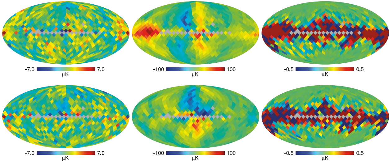
Fig. 1.— Low resolution polarized Q (top) and U (bottom) maps of the CMB, synchrotron, and dust emission, estimated from the five-year K, Ka, Q, and V band maps using Gibbs sampling. Pixels inside the processing mask are grey. The CMB maps (left panels, thermodynamic temperature) do not show significant Galactic contamination in the plane. The synchrotron amplitudes (center, antenna temperature), are defined at K-band (22.8 GHz), and are consistent with the total K-band maps, with high Q and U emission from the North Polar Spur, and high Q emission in the Galactic plane at longitude 110 \lesssim l \lesssim 170 . The dust amplitudes (right, antenna temperature) are defined at W-band (93.5 GHz), and have a prior that bounds P = \sqrt{Q^2 + U^2} to be less than 20% of the dust intensity in each pixel.
