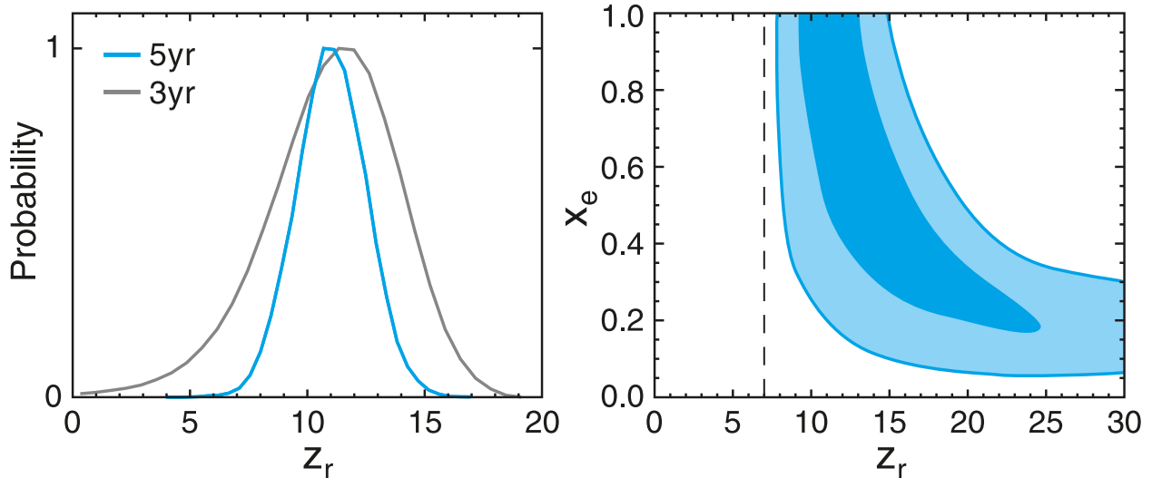
Fig. 8.— Left: Marginalized probability distribution for z_{\text{reion}} in the standard model with instantaneous reionization. Sudden reionization at z = 6 is ruled out at 3.5\sigma , suggesting that reionization was a gradual process. Right: In a model with two steps of reionization (with ionization fraction x_e at redshift z_r , followed by full ionization at z = 7 ), the WMAP data are consistent with an extended reionization process.
